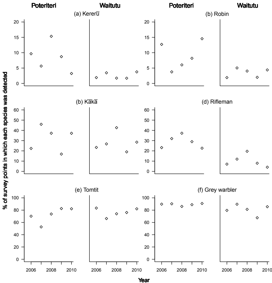
Figure 3. Annual variations in the percentage of five-minute count points at which kererū, robins, kākā, riflemen, tomtits and grey warblers were detected for November surveys at Poteriteri and Waitutu between 2006 and 2010. Application of 1080 baits occurred on 4 and 5 October 2010. Note that the vertical scales change between species.
